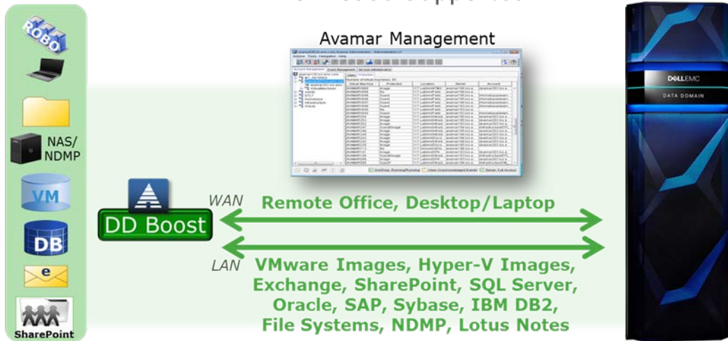
Figure 4: DD Boost for Avamar
