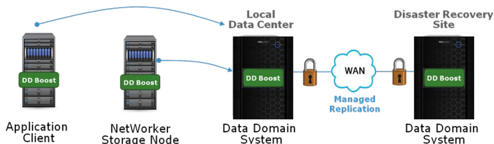
Figure 5: DD Boost for NetWorker
