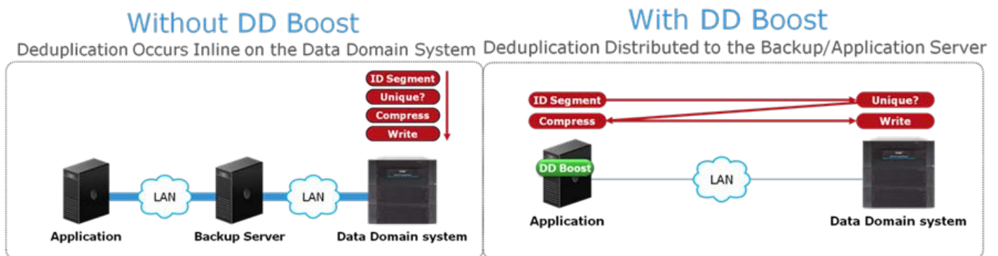
Figure 1: DD Boost distributed segment processing
