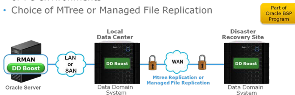
Figure 7: DD Boost for Oracle RMAN
