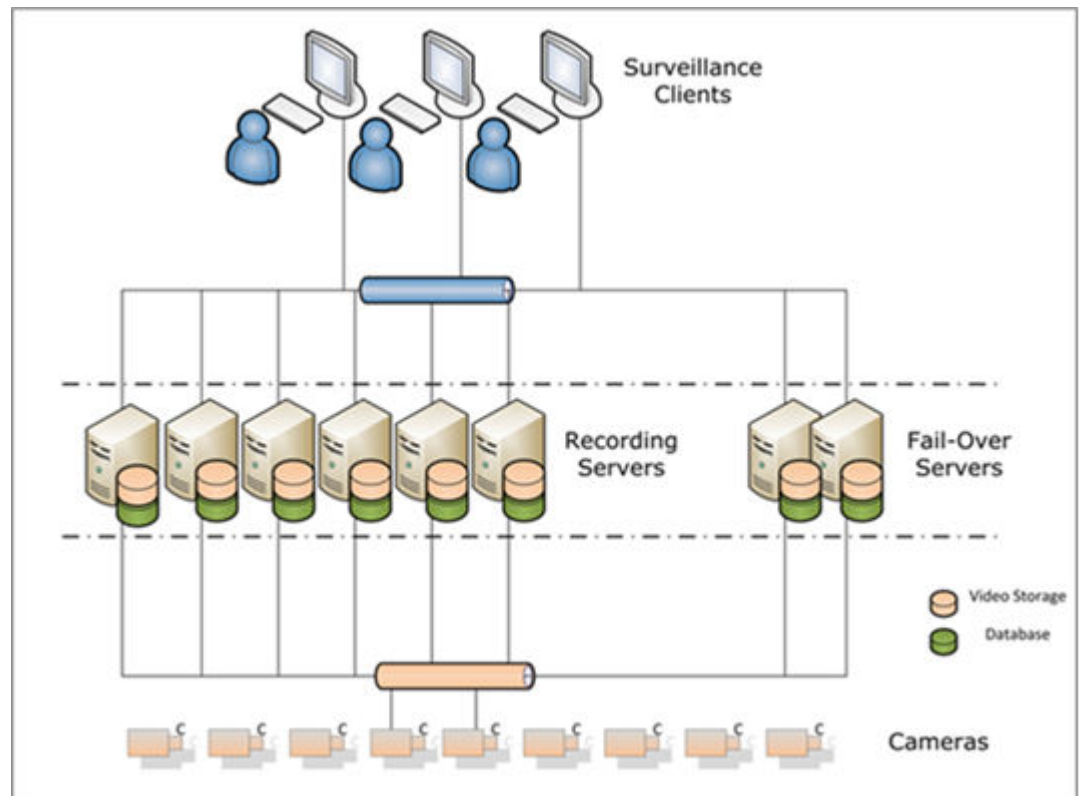
Figure 1 Digifort Enterprise architecture
