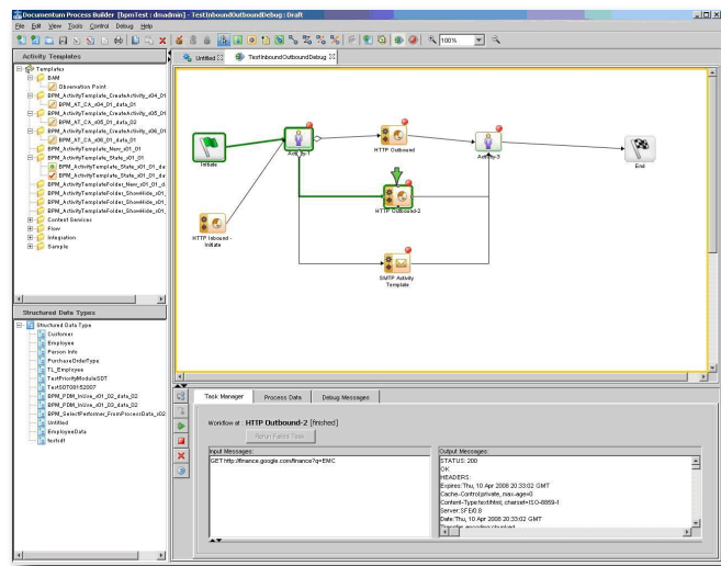
Process Debugger
