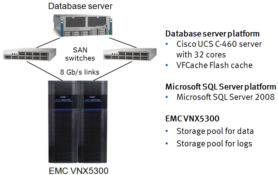
Figure 5. EMC VFCache with Microsoft SQL Server and VNX5300
